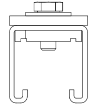
Mounting closed side ( 1 : 2 )
