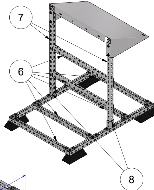
Back View ( 1/20 )
